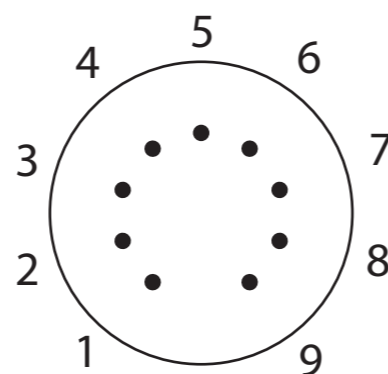
Noval
