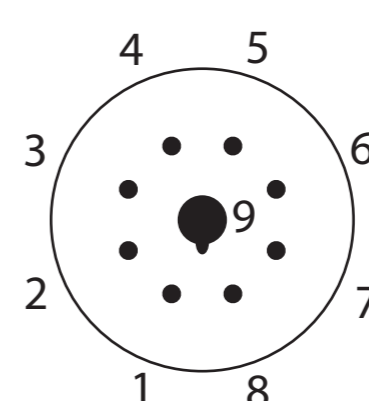
Loktal-8-Stift
